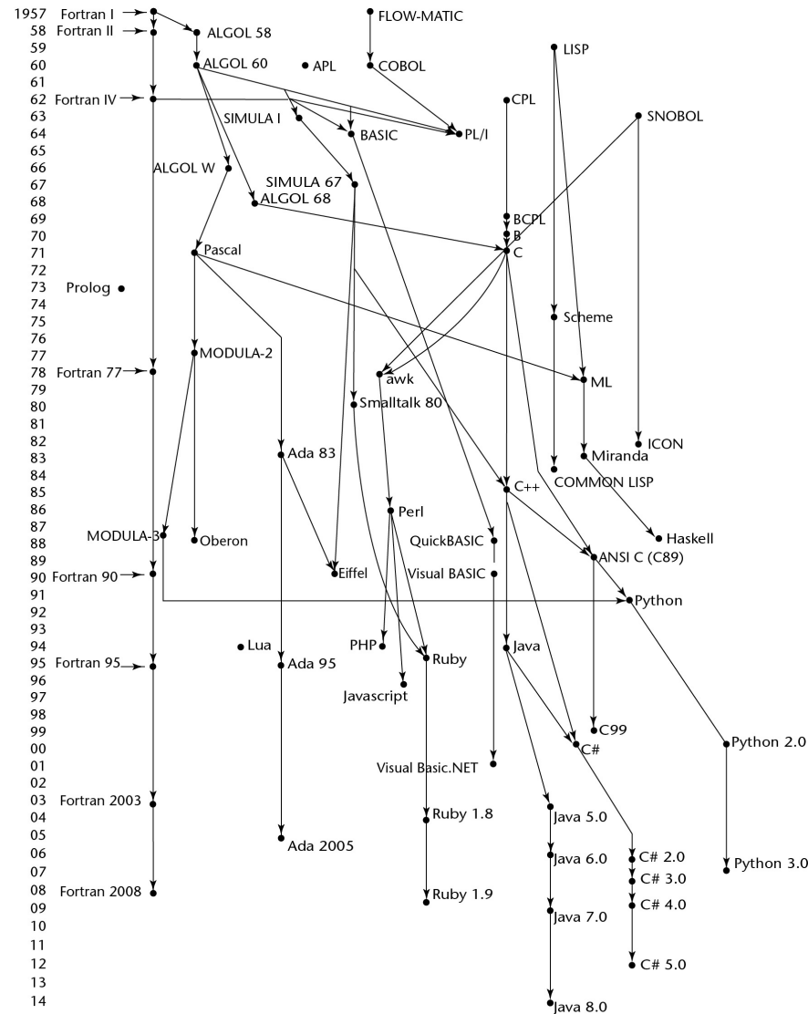
Figure 2.1 Genealogy of common high-level programming languages
